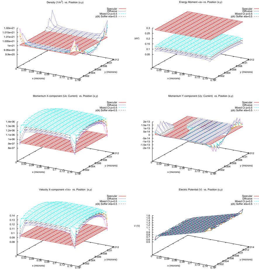
Figure 6.4: Density \rho ( m^{-3} ), Mean energy e ( eV ), Momentum U_x, U_y ( 10^{28} \frac{cm^{-2}}{s} ), Average Velocity Component V_x , and Potential V (Volts) vs Position (x, y) in ( \mu m ) plot for Specular, Diffusive, Mixed p = 0.5 & Mixed p(\vec{k}) = \exp(-4\eta^2 |k|^2 \sin^2 \varphi) , \eta = 0.5 Reflection for electrons in 2D bulk silicon with reflective BC in y and periodic BC in x .
