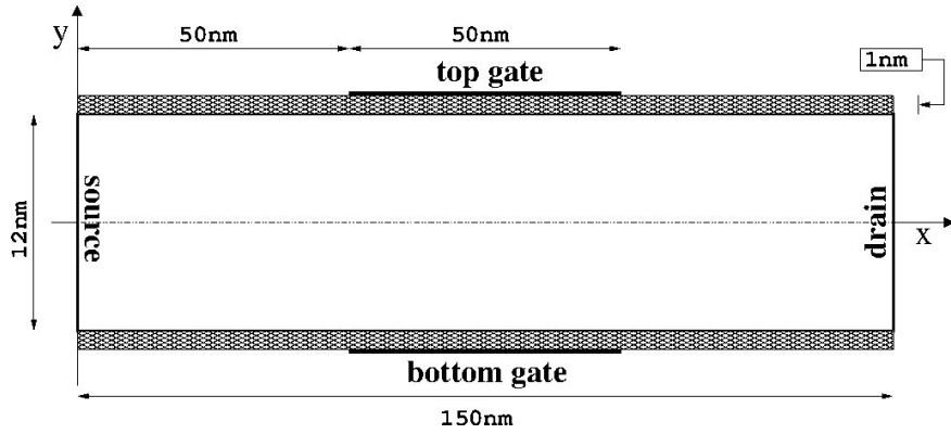
Figure 4.1: Schematic representation of a 2D double gate MOSFET device. From Y. Cheng, I. M. Gamba, A. Majorana and C.-W. Shu, 'A discontinuous Galerkin solver for Boltzmann Poisson systems in nano devices', Computer Methods in Applied Mechanics and Engineering, v198 (2009), p. 3143.
