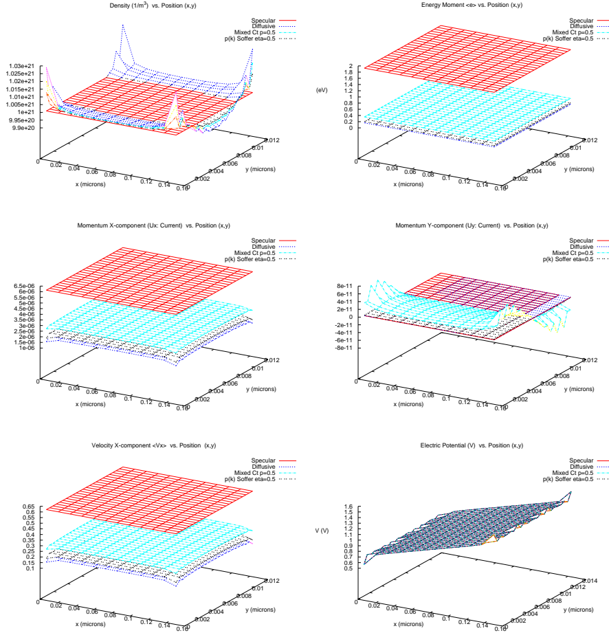
Figure 6.5: Density \rho ( m^{-3} ), Mean energy e ( eV ), Momentum U_x, U_y ( 10^{28} \frac{cm^{-2}}{s} ), Average Velocity Component V_x , and Potential V (Volts) vs Position (x, y) in ( \mu m ) plot for Specular, Diffusive, Mixed p = 0.5 & Mixed p(\vec{k}) = \exp(-4\eta^2|k|^2 \sin^2 \varphi) , \eta = 0.5 Reflection for 2D collisionless electrons with reflective BC in y and periodic BC in x .
