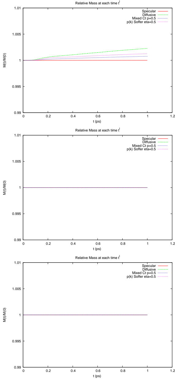
Figure 6.6: Relative Mass vs Time (ps) plot for Specular, Diffusive, Mixed p = 0.5 & Mixed p(\vec{k}) = \exp(-4\eta^2|k|^2 \sin^2 \varphi) , \eta = 0.5 Reflection. The figure on top is related to the simulations for bulk silicon with charge neutrality conditions on the non-reflecting boundaries. The figure in the middle is associated to the simulations for bulk silicon with periodic boundary conditions on the non-reflecting boundaries. The bottom figure is related to the simulations for collisionless electron transport with periodic boundary conditions on the non-reflecting boundaries. The figures show the conservation of mass when isolating the effect of reflection boundary conditions in the simulations, as the slight increase in the relative mass of less than 0.5% is associated only to simulations that also include charge neutrality conditions and possibly an accumulation of numerical error due solely to it.
