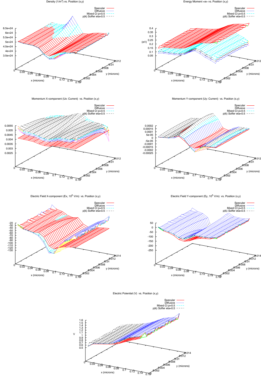
Figure 6.3: Density \rho ( m^{-3} ), Mean energy e (eV), Momentum U_x, U_y ( 10^{28} \frac{cm^{-2}}{s} ), Electric Field Components E_x and E_y , and Potential V (Volts) vs Position (x, y) in ( \mu m ) plot for Specular, Diffusive, Mixed p = 0.5 & Mixed p(\vec{k}) = \exp(-4\eta^2|k|^2 \sin^2 \varphi) , \eta = 0.5 Reflection for a 2D double gated MOSFET.
