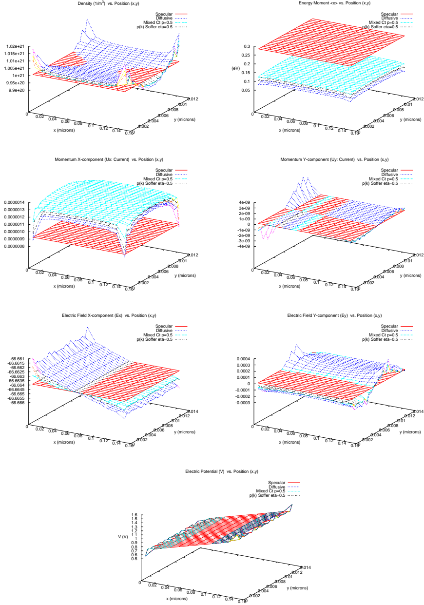
Figure 6.2: Density \rho ( m^{-3} ), Mean energy e (eV), Momentum U_x, U_y ( 10^{28} \frac{cm^{-2}}{s} ), Electric Field Components E_x and E_y , and Potential V (Volts) vs Position (x, y) in ( \mu m ) plot for Specular, Diffusive, Mixed p = 0.5 & Mixed p(\vec{k}) = \exp(-4\eta^2 |k|^2 \sin^2 \varphi) , \eta = 0.5 Reflection for 2D bulk silicon.
